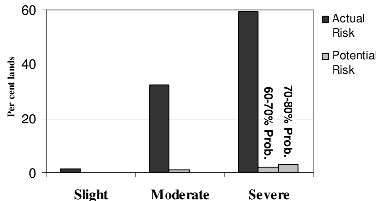
Figure 4. Percent land under different risk classes of vegetation degradation in the Payab basin.
