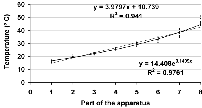
Figure 1. Temperature gradient in different parts of an apparatus modeled after that of Weseloh (1971). Points show the observed data while the lines show linear and exponential predictions of the same data
