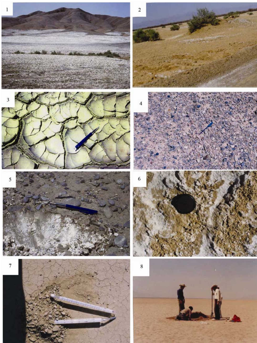
Figure 3. Surface conditions of training classes: (1) Salt crust; (2) Puffy soil; (3) Polygon crust; (4) Gravely soil; (5) Gravely soil with gypsum; (6) Saline soil affected by calcium and magnesium chloride; (7) Sealing, (8) Very severely saline soil.
