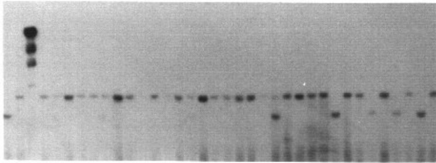
Figure 5. Segregation pattern of double haploid lines (DHIS) in IR64 (I) /Azucena (A) cross (Huang et al. , 1994), using RAPD marker (AG8-AR) via Southern analysis when digested with TaqI . M= molecular weight marker ( \lambda / HindIII ). Lower band indicates Azucena allele and upper band indicates IR64 allele.
