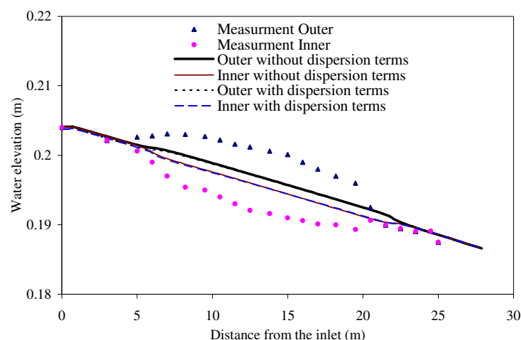
Figure 2. Comparison between sidewall flow depth, ignoring and taking secondary flow into account; mildly curved channel.
