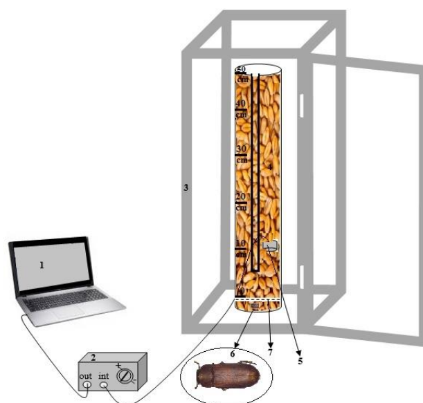
Figure 2. The soundproof test rig including: (1) PC; (2) Integrated signal detection and processing; (3) Acoustic insulation chamber; (4) Grain cylindrical graded repository; (5) Acoustic sensor; (60) Tribolium confusum , (7) Thin grid.
