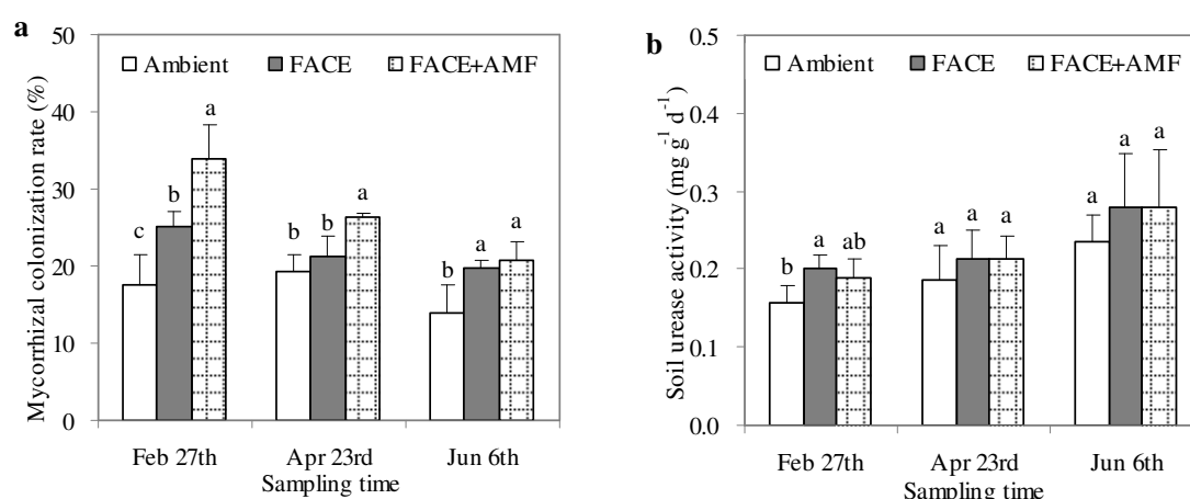
Figure 1. Mycorrhizal colonization rate (a) and soil urease activity (b) with or without arbuscular mycorrhizal fungi (AMF) inoculation under elevated surface [O 3 ]. Vertical T bars indicate standard deviations. Bars not topped by the same letter within the same sampling time indicate a significant difference in values ( P < 0.05 ).
