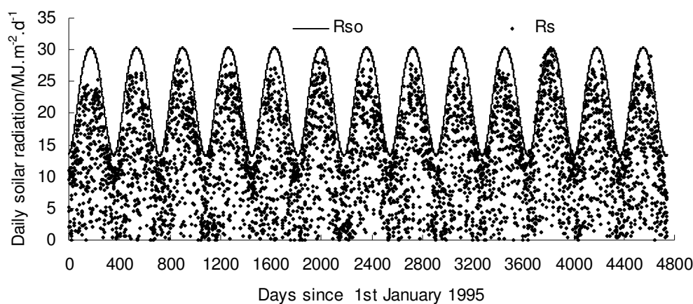
Figure 1. Comparison between daily solar radiation ( R_s ) and clear sky radiation ( R_{so} ).
