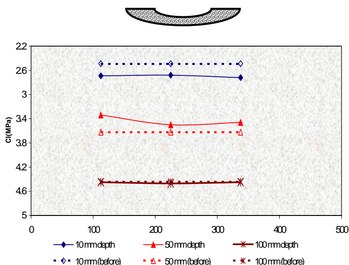
Figure 7. The penetration resistance under a single tyre in the firm field.
