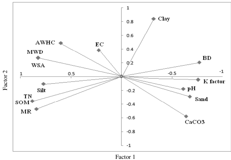
Figure 2. Loading plot indicating associations of soil properties to Factors 1 and Fcator 2 in the area studied.
