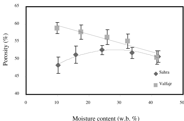
Figure 6. Effect of moisture content on porosity of barley kernels.
