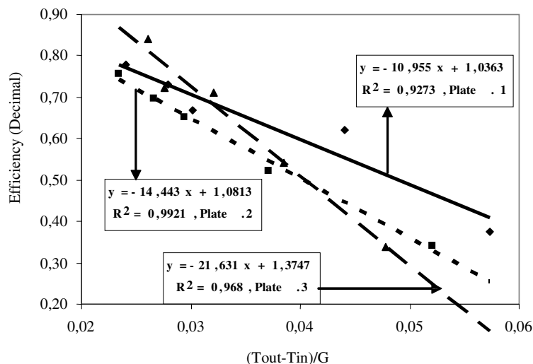
Figure 7. Variations of normalized air temperatures, [(T_{out}-T_{in})/G, (°C m^2 W^{-1})] , vs. collector efficiency for three absorber plates.
