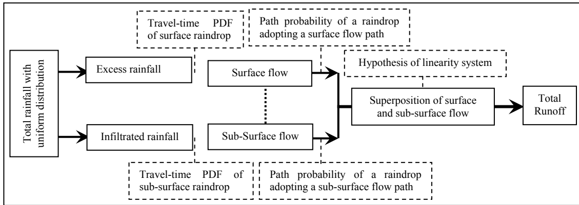
Figure 2. Flow diagram of surface and subsurface flows in GIUH theory.
