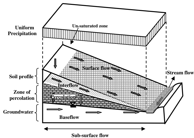
Figure 1. Interaction between surface, sub-surface and interflow.
