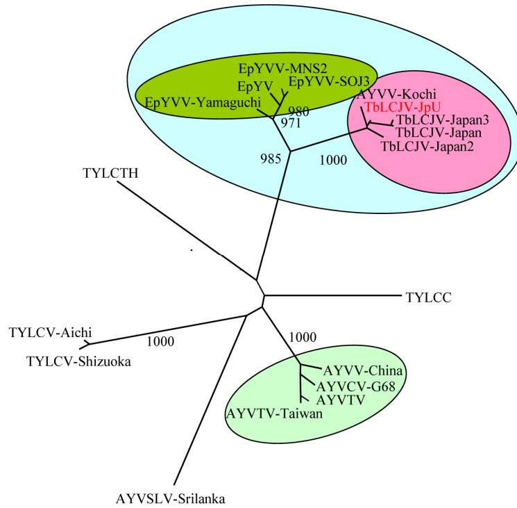
Figure 2. Phylogenetic relationship in aa sequence of CP of TbLCJV-JpU isolate, with TbLCJV, TYLCV, EpYVV and AYVV isolates reported in the GenBank, using neighbour joining method with a bootstrap value of 1,000.
