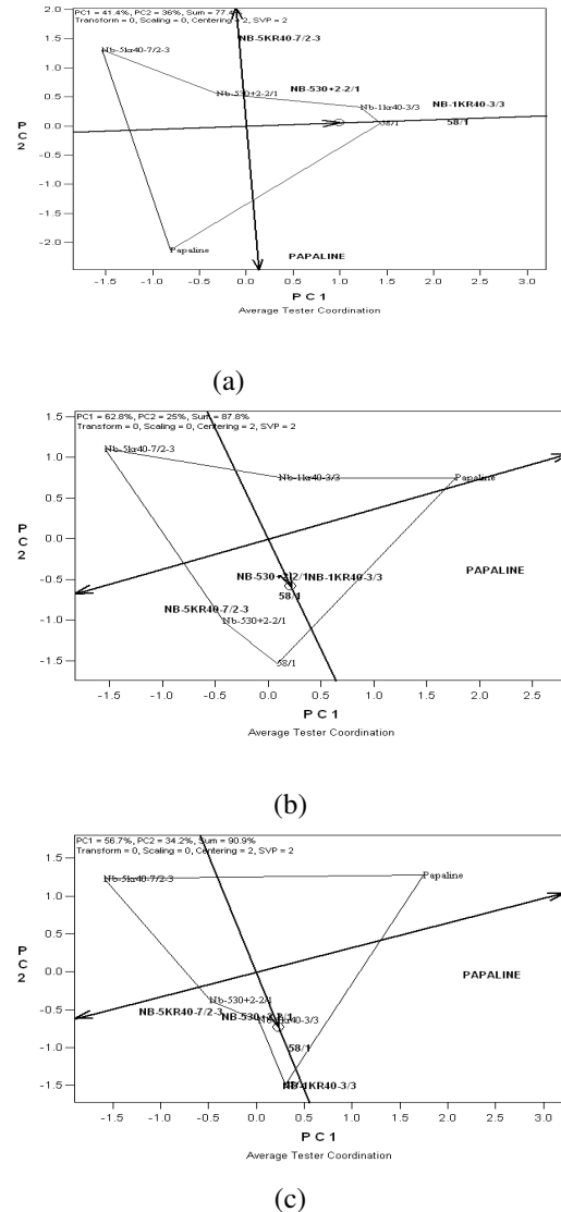
Figure 4. Polygon view of biplot for narcotine: (a) Straight F 1 ; (b) Reciprocal F 1 , (c) Removing reciprocal differences F 1 .
