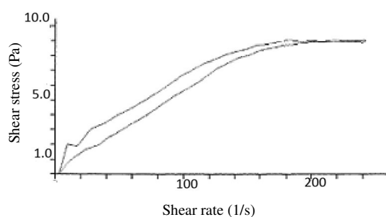
Figure 11. Thixogram of the chocolate beverage of Brazilian market (Sample H) at 25°C.
