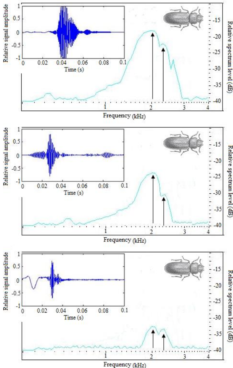
Figure 5. The acoustic characteristics of the adult insect of Tribolium confusum recorded within wheat grain mass at different distances of insect and audio sensor (from top to bottom 10, 20 and 30 cm, respectively).
