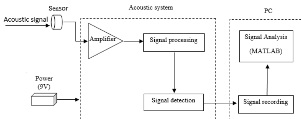
Figure 1. Flow diagram for acoustic signal detection and signal analysis of insect pests within a grain bulk.
