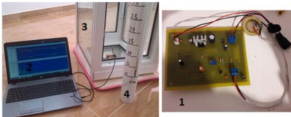
Figure 3. The laboratory equipment: (1) Integrated signal receive and amplify (acoustic sensor); (2.) PC; (3) Acoustic insulation chamber, (4) Graded container.
