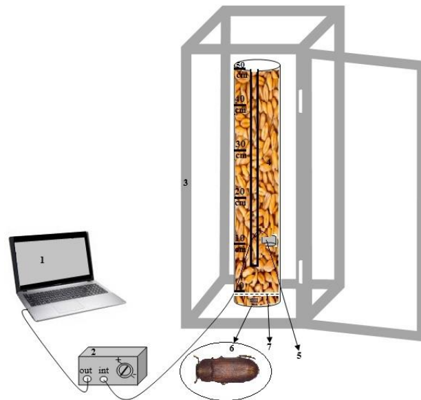
Figure 2. The soundproof test rig including: (1) PC; (2) Integrated signal detection and processing; (3) Acoustic insulation chamber; (4) Grain cylindrical graded repository; (5) Acoustic sensor; (6) Tribolium confusum , (7) Thin grid.
