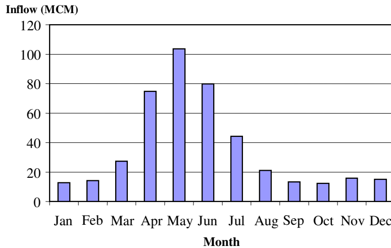
Figure 2. Average monthly inflow to Amir-Kabir dam.
