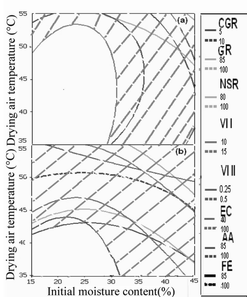
Figure 12. The optimum drying conditions for soybean seeds after overlaying the contour plots in: (a) Clark and (b) Sahar cultivars.
