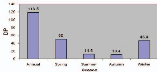
Figure 4. Annual and seasonal drift potential (in VU) (1986-2005). Drift potential (DP).
