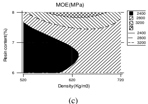
Figure 2. Modulus of elasticity ( MOE ) counter plot for (a) poplar panels, (b) Beech panels (c) Hornbeam panels.
