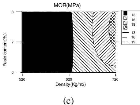
Figure 1. Modulus of rupture ( MOR ) counter plot for (a) poplar panels (b) Beech panels (c) Hornbeam panels.
