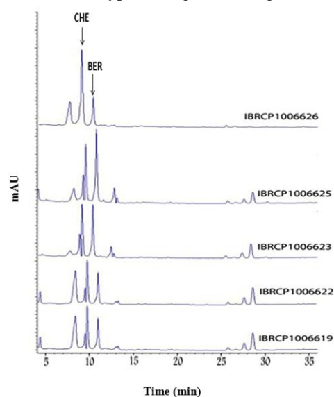
Figure 4. Separated chelidone and berberine chromatograms from leaves of five Iranian C. majus ecotypes at vegetative stage.
